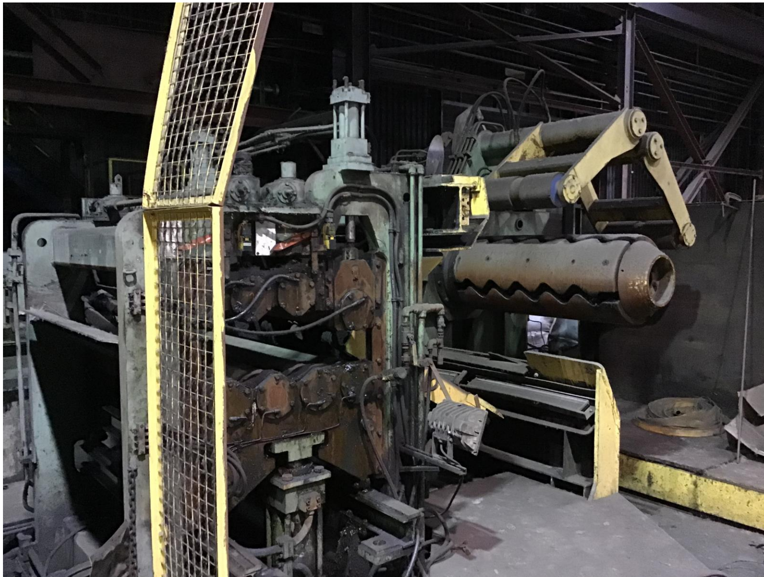
PAYOFF REEL: 24" DIA MANDREL (610mm) 160HP MOTOR DC (120Kw) 770 / 2300RPM – 400v
